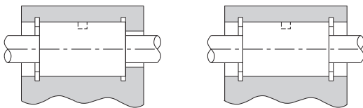
止动环
