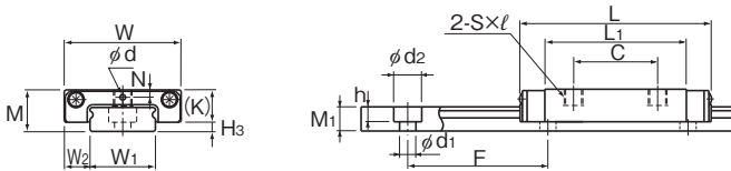
RSR3~7WM/WN型
